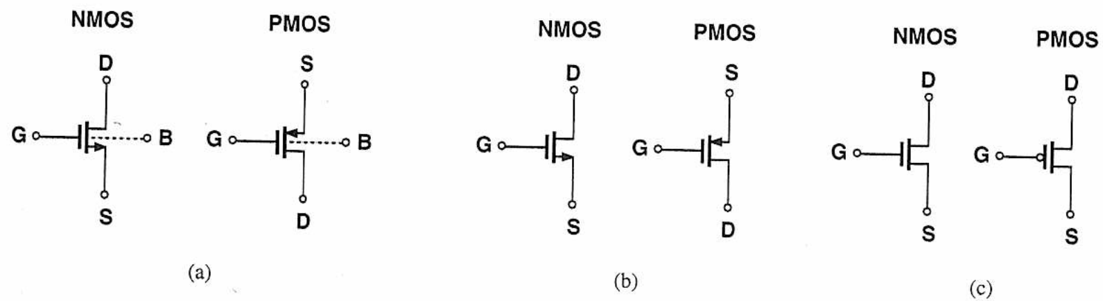
Figure 2.5 MOS symbols.
