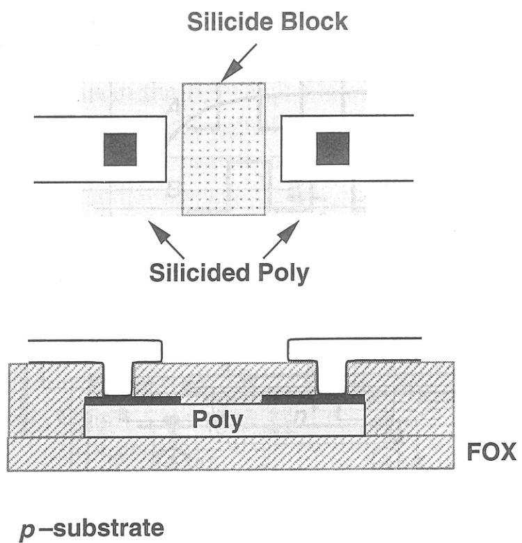
Figure 17.13 Poly resistor using silicide block.
